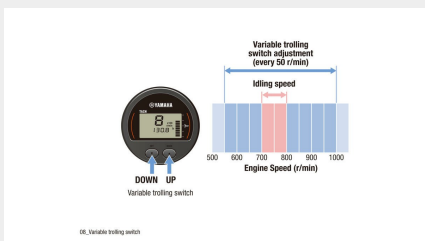
04, Variable trolling switch
