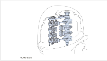
11, SOHC 16 valves
